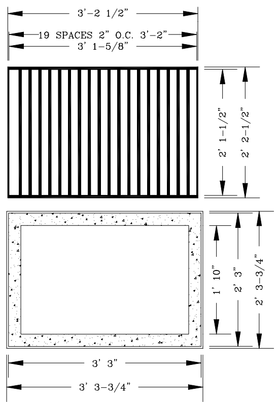
FRAME AND GRATE DETAIL
