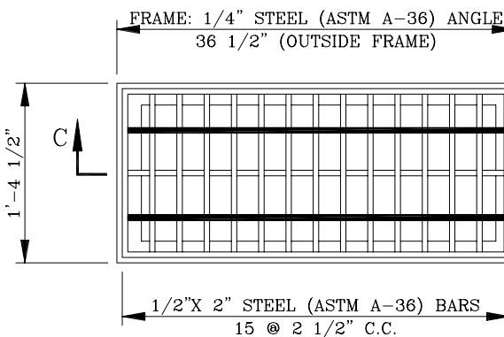
WELDED STEEL FRAME AND GRATE PLAN
