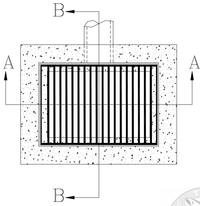
FRAME AND GRATE DETAIL
