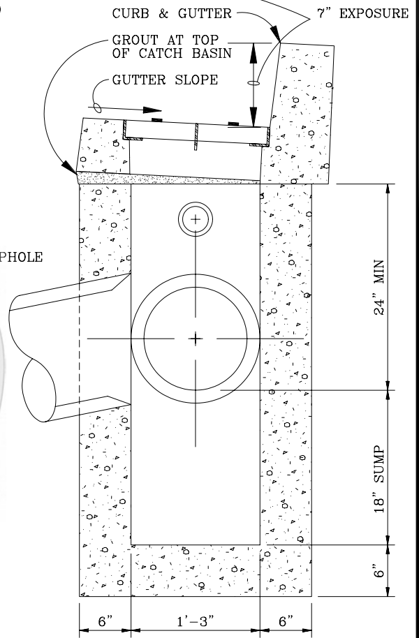
SECTION B-B
